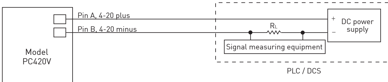
Typical circuit
